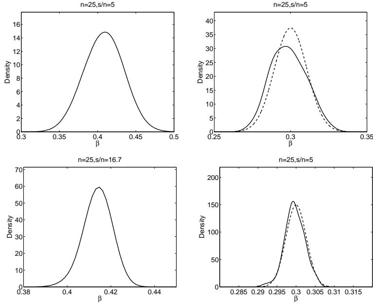
Figure 6: Simulated (solid curve) and asymptotic (dashed curve) distributions of \hat{\beta}_{\Delta, N} for f_2 (left panels) and f_3 (right panels). The variance of the asymptotic distributions is given as \frac{8\sigma^2\Delta^2}{M_N''(\beta^*)} (cf. Theorem 3). The parameter N was chosen as 7, except for the lower left where it was chosen as 8.
